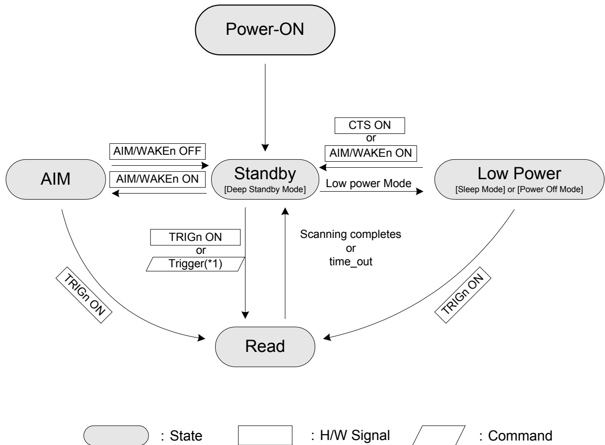
Figure 3: Power Mode Transition
